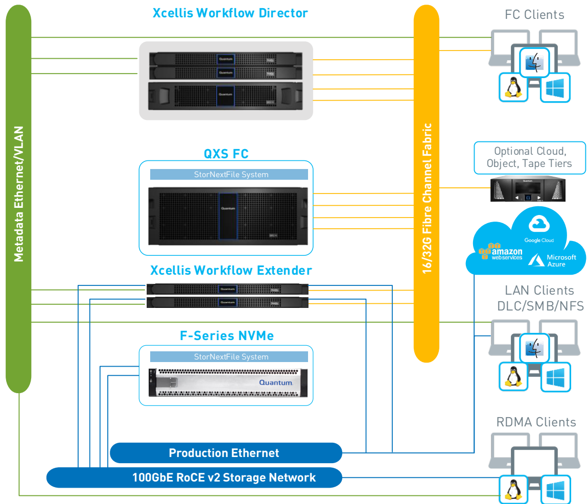
Figure 7 – Mixed Fibre Channel & Ethernet Reference Architecture
