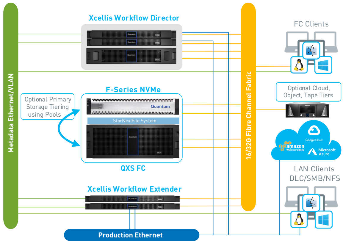
Figure 5 – Fibre Channel Reference Architecture
