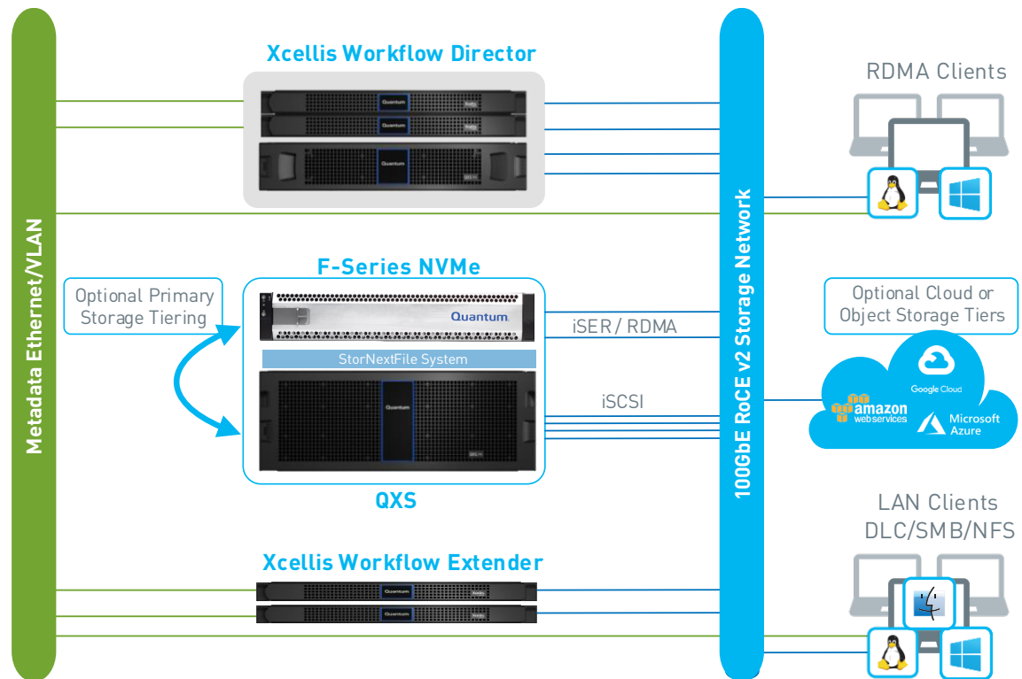
Figure 6 – Ethernet Reference Architecture
