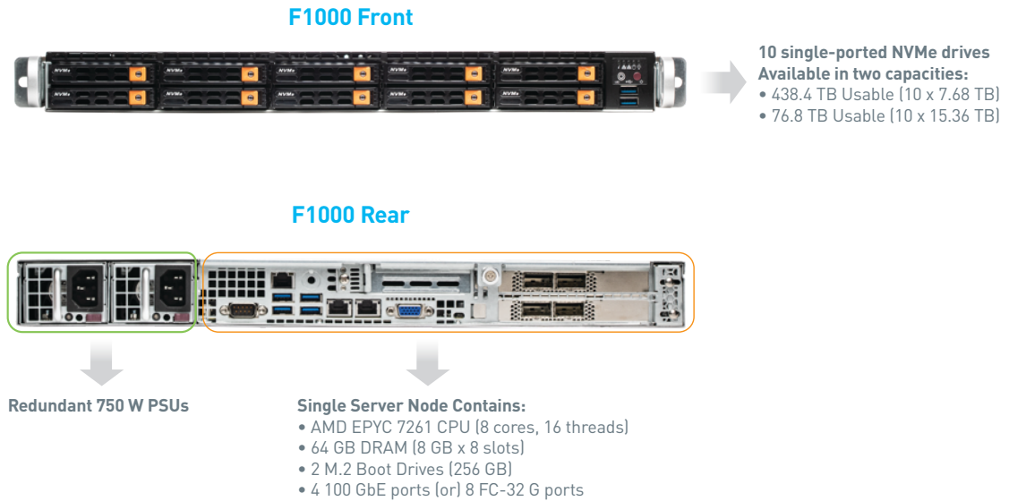
Figure 2 – F1000 Hardware Overview
