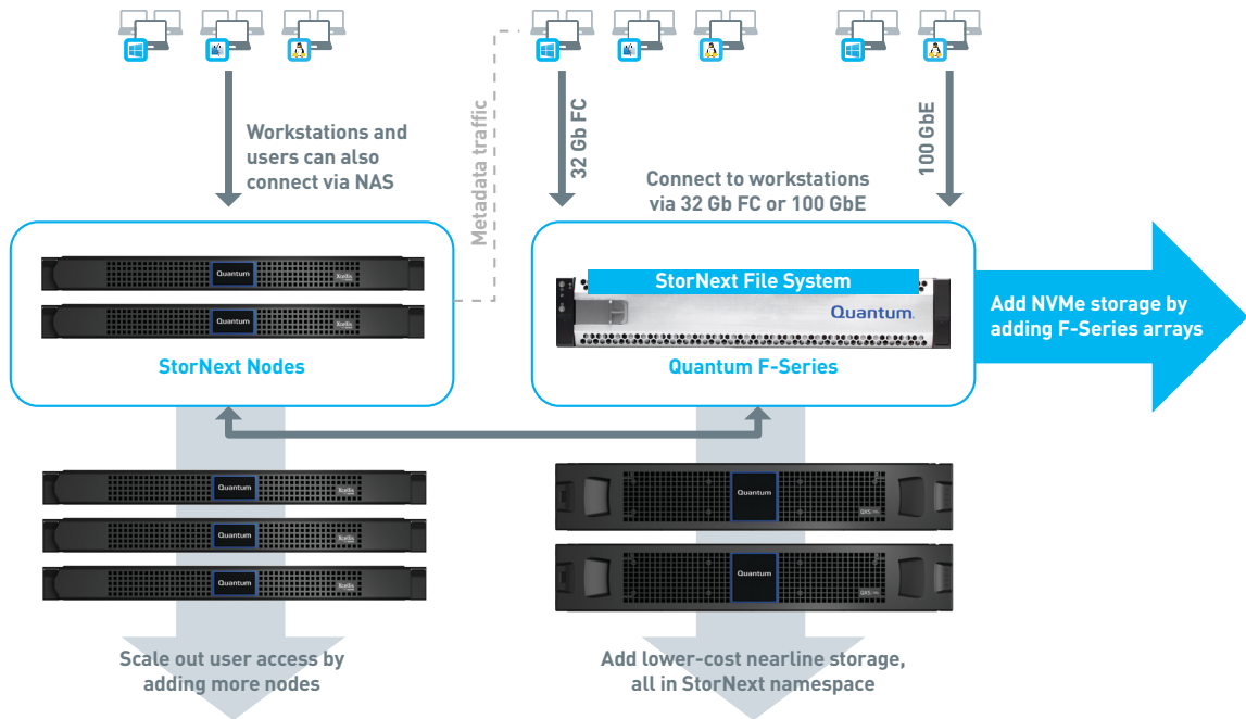
Figure 3 – Scaling Model
