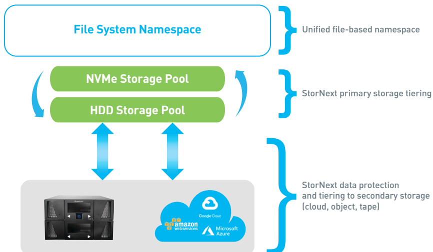
Figure 4 – StorNext Tiering
